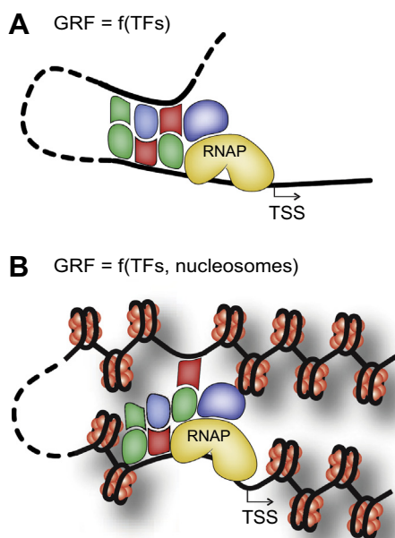
Fig. 1. Different levels of cis -regulatory module functioning. (A) Enhancer and promoter regions can be connected by a DNA loop bridged by transcription factors. One of the bound proteins is RNA polymerase (RNAP), whose binding determines the probability of transcription initiation. (B) In chromatin, both enhancer and promoter regions might be covered by nucleosomes; some nucleosomes need to be removed or repositioned to be compatible with TF binding, which becomes an additional layer of regulation of the initiation of transcription.
